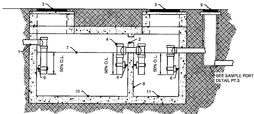
ELEVATION VIEW
